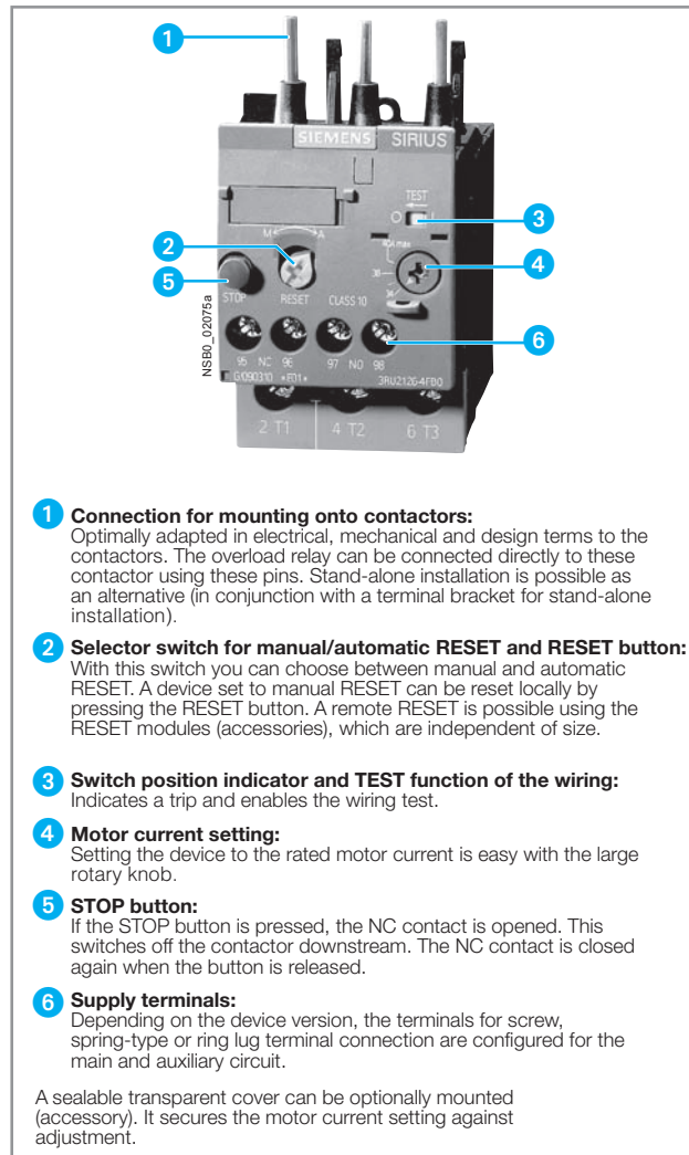
3RU21 26-4FB0 thermal overload relays
